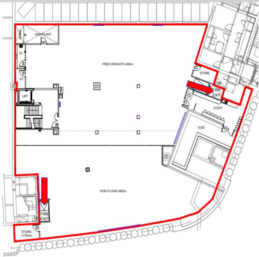
BASEMENT MEZZANINE FLOOR
